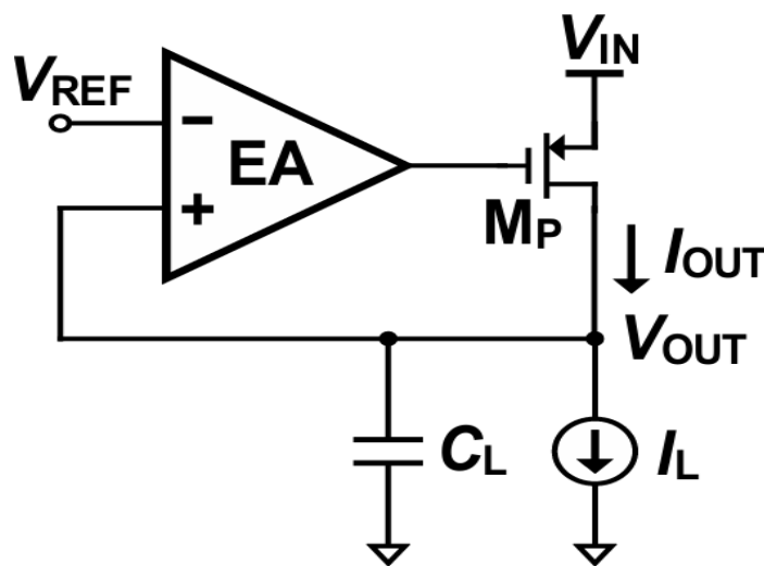
Figure 1.2 Basic structure of an LDO
